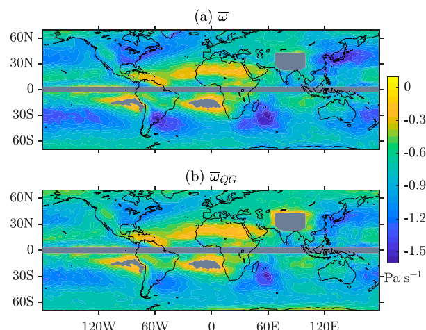
FIG. 3. (a) \bar{\omega} and (b) \bar{\omega}_{QG} , both in Pa s -1 , at 500 hPa associated with precipitation extremes in the historical simulations with CESM-LE. Masking and smoothing are as in Fig. 2.
